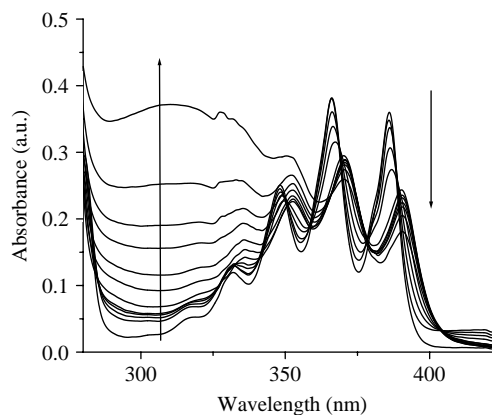
Figure 9. Change in absorbance of 1 ( c = 4.10 \times 10^{-5} M) upon gradual addition of Cu 2+ ion.
