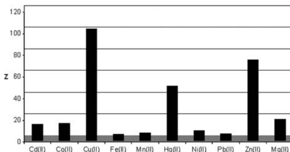
Figure 5. Fluorescence enhancement factor ( Z ) of receptor 1 ( c = 4.10 \times 10^{-5} M) upon addition of 15 equiv. amounts of various metal ions.
