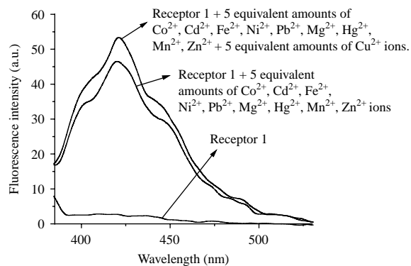
Figure 6. Change in emission of receptor 1 ( c = 4.10 \times 10^{-5} M) upon addition of Cu^{2+} in the presence of other metal ions.
