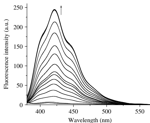
Figure 2. Change in emission of 1 ( c = 4.10 \times 10^{-5} M) upon gradual addition of Cu(ClO 4 ) 2 .
