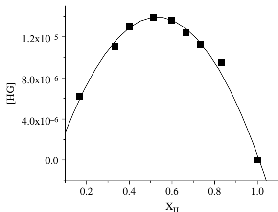
Figure 4. UV-vis job plot for receptor 1 ( [H] = [G] = 4.45 \times 10^{-5} M) with Cu^{2+} at 365 nm.
