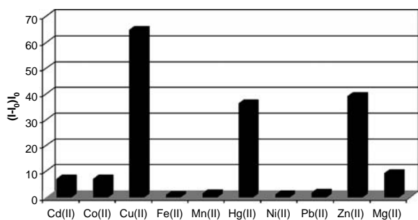
Figure 1. Change in fluorescence ratio of 1 ( c = 4.10 \times 10^{-5} M) upon addition of 15 equiv. amounts of cations at 418 nm.
