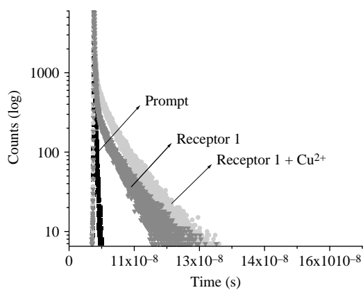
Figure 7. Fluorescence decays (at \lambda_{\max} = 418 nm) of receptor 1 upon addition of 1 equiv. of Cu(ClO 4 ) 2 ( [H] = 4.10 \times 10^{-5} M, [G] = 8.21 \times 10^{-4} M) in CH 3 CN containing 0.04% DMSO.
