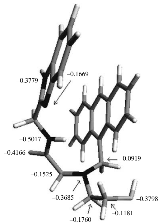
Figure 11. AM1 optimised geometry of 1 in gas phase ( E = -194.067 au; the closest distance between anthracene and benzimidazole is 4.89 Å).
