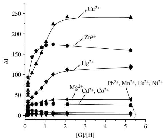
Figure 3. Fluorescence titration curves ( [guest]/[host] vs. change in emission) of 1 ( c = 4.10 \times 10^{-5} M) measured at 418 nm in CH_3CN containing 0.04% DMSO.
